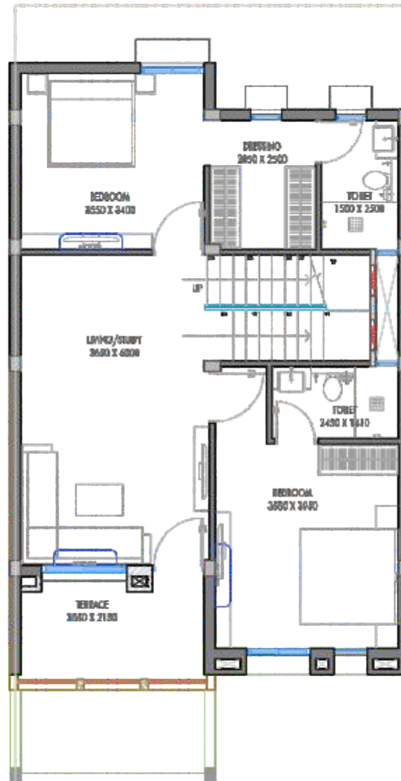
FIRST FLOOR
