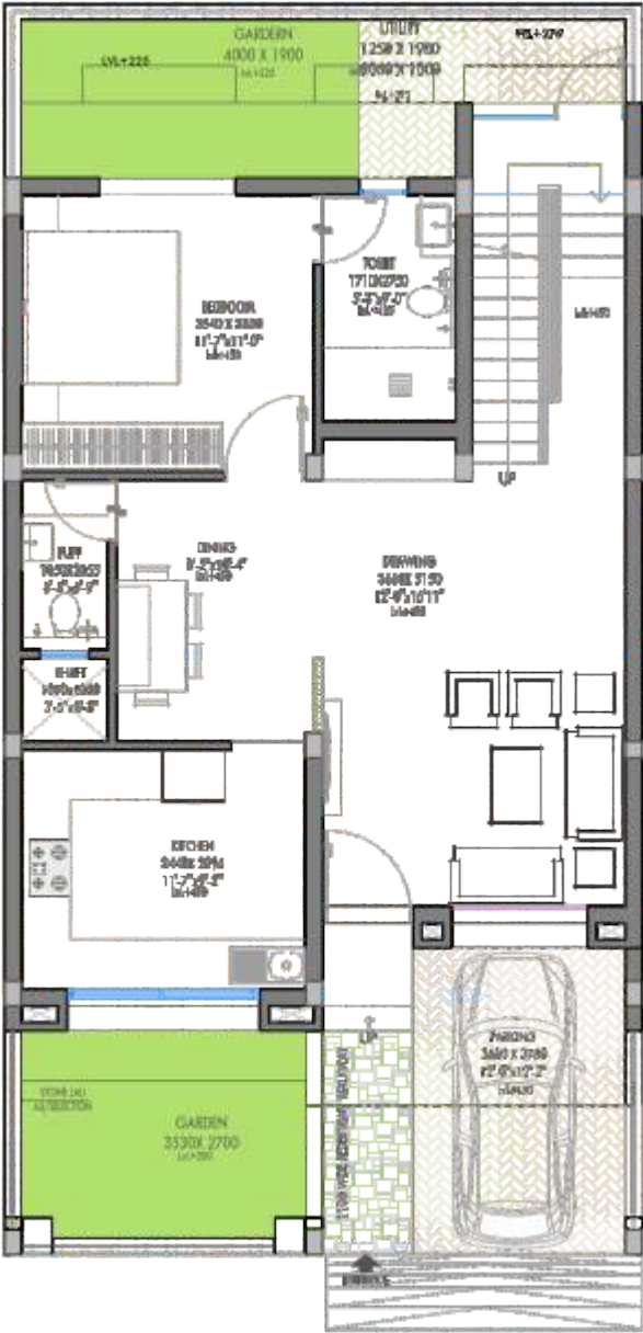
GROUND FLOOR
